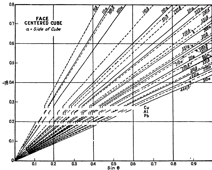
FIG. 19.—Owen and Preston's chart for face-centered cubic lattice.
